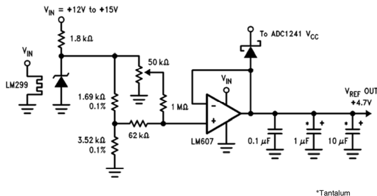
FIGURE 2. Low Drift Extremely Stable Reference Circuit
